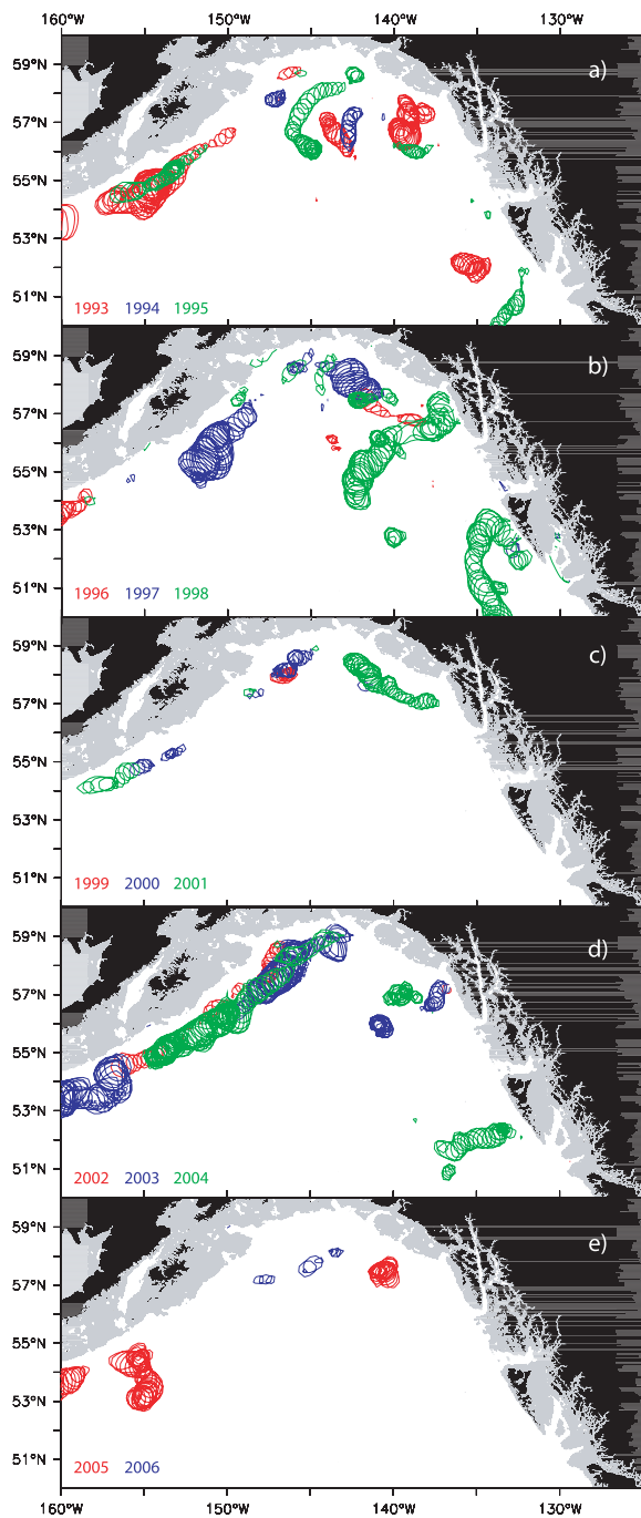
Figure 3. (a–e) Contours of 25 cm SLA colored by the years indicated. The year 2006 includes data through May.
