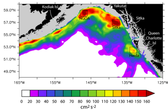
Figure 1. Mean EKE ( \text{cm}^2 \text{s}^{-2} ). Gray region is shelf (<300 m depth).
