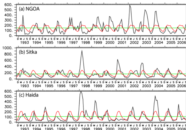
Figure 2. Time series of monthly averaged (black), monthly climatological (red), and mean (green) EKE ( \text{cm}^2 \text{ s}^{-2} ) averaged over the three boxes shown in Figure 1. (a) NGOA, (b) Sitka, and (c) Haida.
